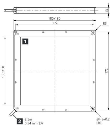
1) Illuminated area 2) Connection cable
