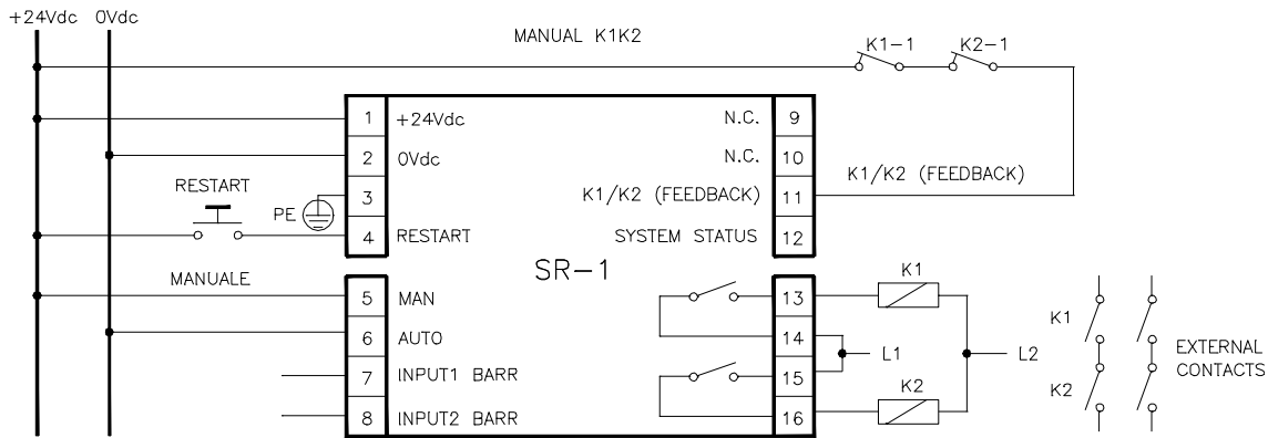
Figure 4 Manual operation with K1/K2 relays
